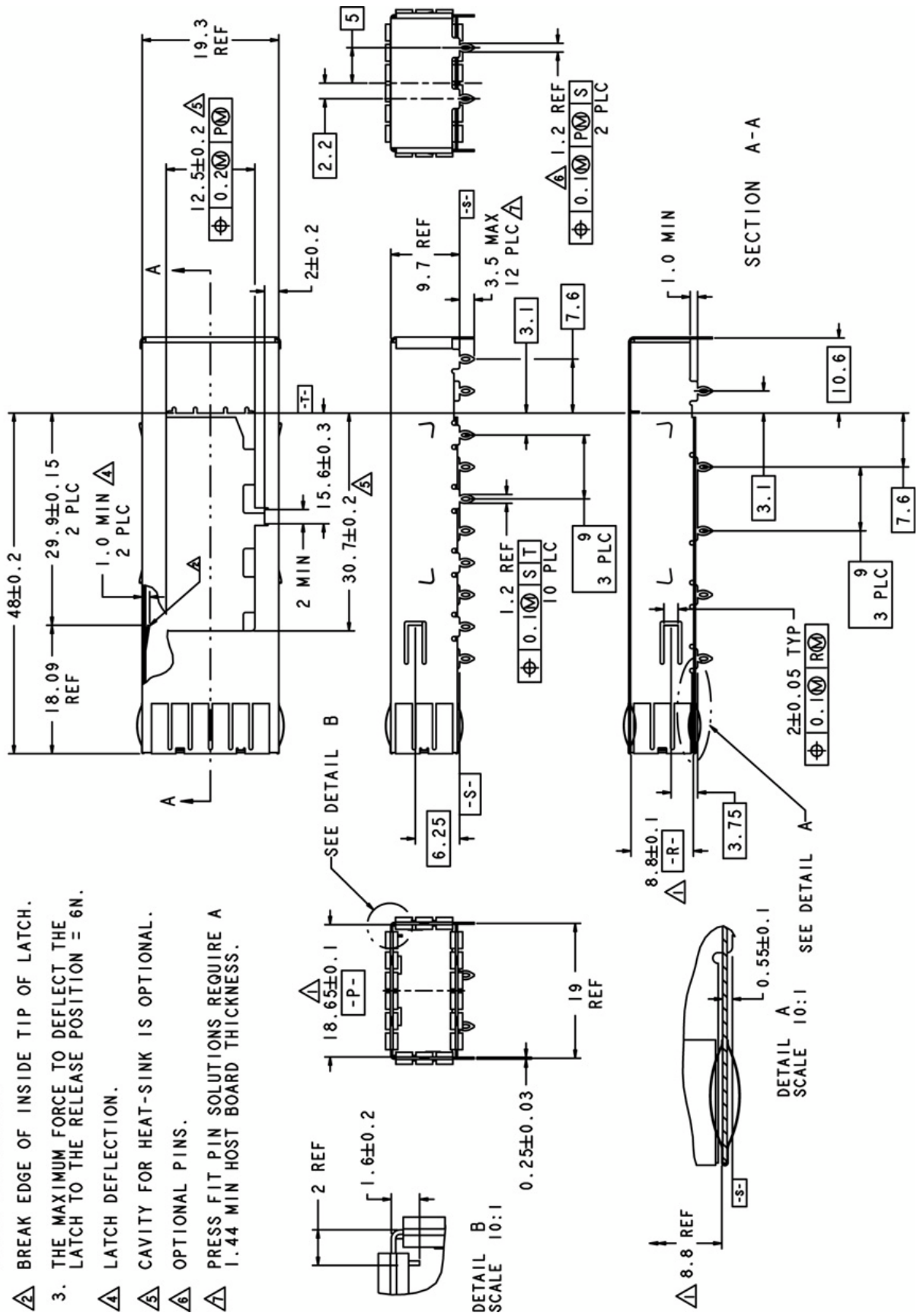
Figure 16 — 1-by-1 cage
