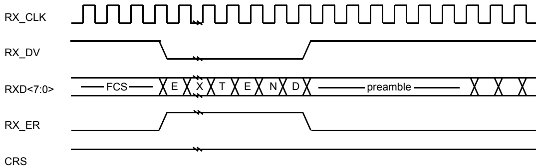
Figure 35-11—Burst reception
