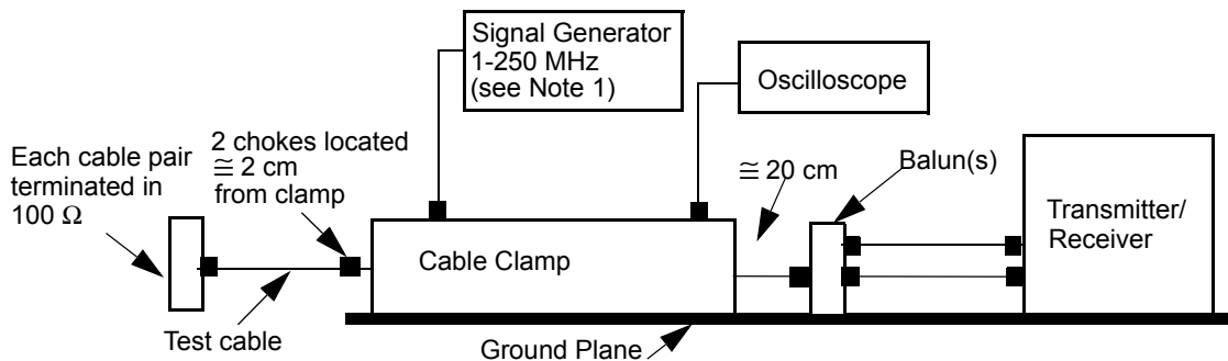
Figure 40B-3—Cable clamp validation test configuration
