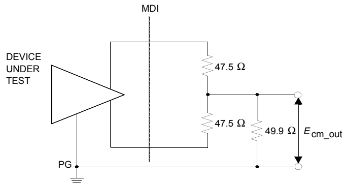
Figure 40-33—Common-mode output voltage test circuit
