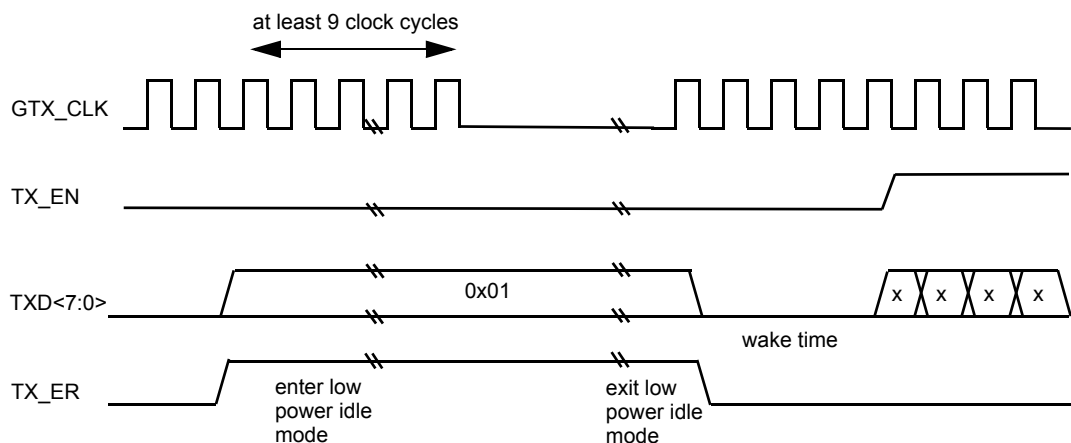
Figure 35-8—LPI transition
