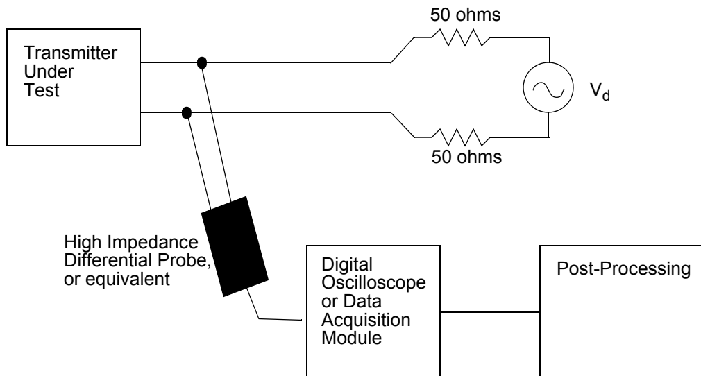
Figure 40–24—Transmitter test fixture 2 for droop measurement
