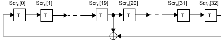
Figure 40–6—A realization of side-stream scramblers by linear feedback shift registers
