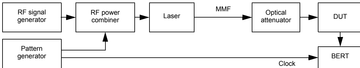
Figure 38-6—Test setup for receiver bandwidth measurement
