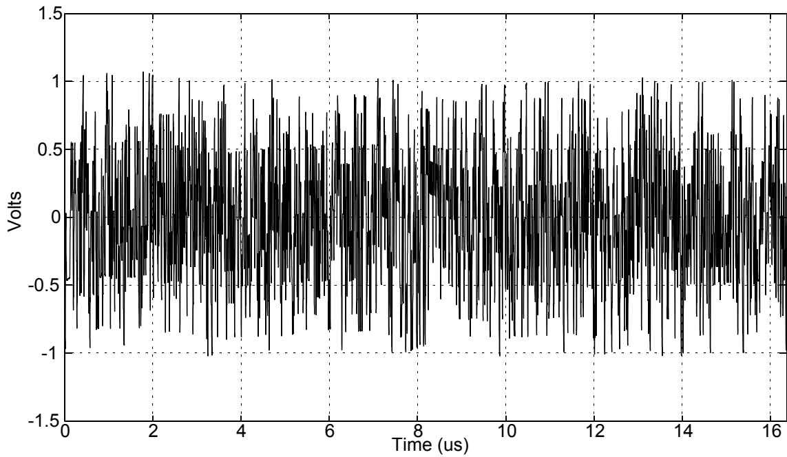
Figure 40-22—Example of Transmitter Test Mode 4 waveform (1 cycle)
