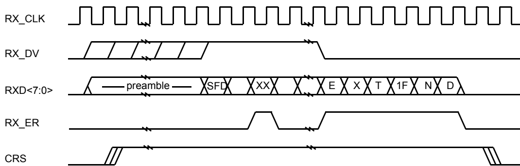
Figure 35–12—Two examples of reception with error
